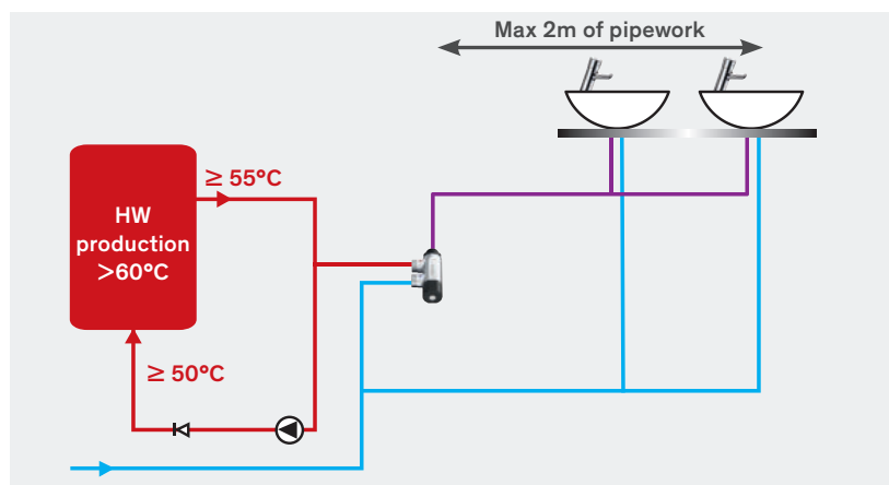
PREMIX COMPACT
